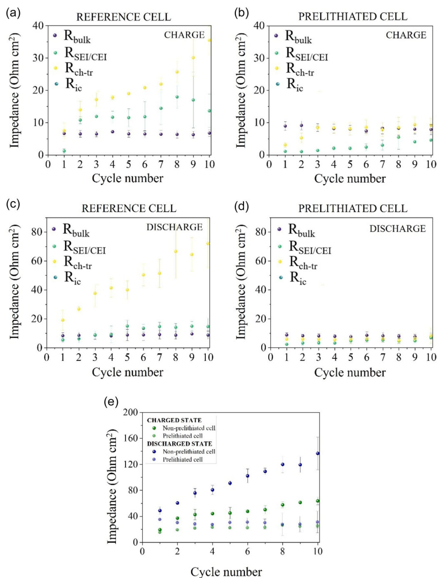
Figure 3. Changes of R_{\text{b}}, R_{\text{SEI/CEI}}, R_{\text{ic}} , and R_{\text{ch-tr}} during the first ten cycles. a) Nonprelithiated cell at charged state, b) prelithiated cell at charged state, c) nonprelithiated cell at discharged state, d) prelithiated cell at discharged state, and e) change of total cell impedance during the initial ten cycles at charge and discharged states. The three Nyquist plots showing the highest consistency out of four repetitions were selected for the calculations.
