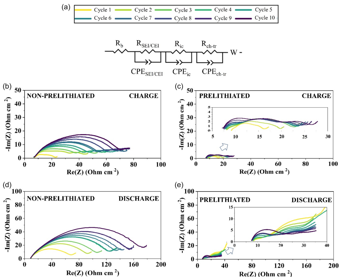
Figure 2. a) Equivalent circuit used to define the NMC-811 || SiGr cells. Nyquist plots showing impedance of the fully charged NMC-811 || SiGr cells during the first 10 cycles for b) nonprelithiated cell and c) prelithiated cell after as well as for fully discharged d) nonprelithiated cell and e) prelithiated cell. (CCCV charge up to 4.2 V and CC discharge down to 2.8 V).
